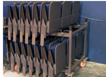
Ranked trolley (alternative to fishbone type).
